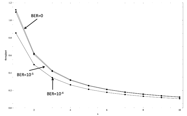
Fig. 3. S_{DATA} as a function of n – for L=214 octets and different values of BER
