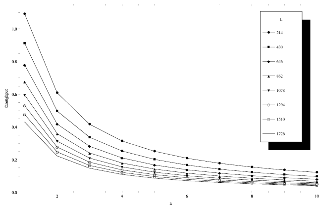
Fig. 5. S_{DATA} as a function of n – for different values of frame length and BER=10^{-5}
