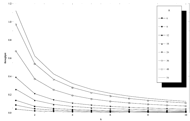
Fig. 7. S_{DATA} as a function of n – for L=214 octets, BER=0 and different values of R
