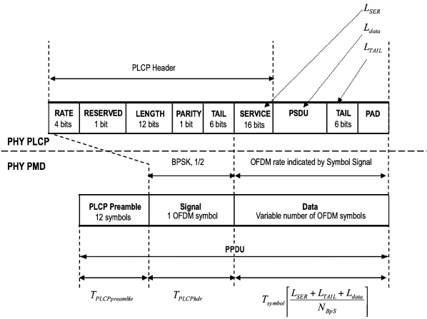
Fig. 1. The structure of 802.11a/g PPDU for ERP-OFDM networks
