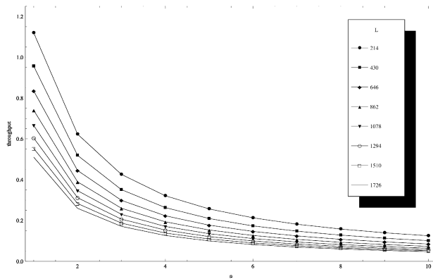
Fig. 4. S_{DATA} as a function of n – for different values of frame length and BER=0
