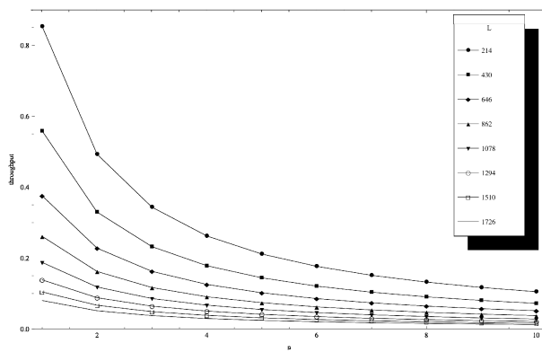
Fig. 6. S_{DATA} as a function of n – for different values of frame length and BER=10^{-4}
