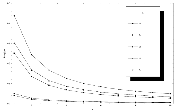
Fig. 8. S_{ACK} as a function of n – for L=214 octets, BER=0 and different values of R
